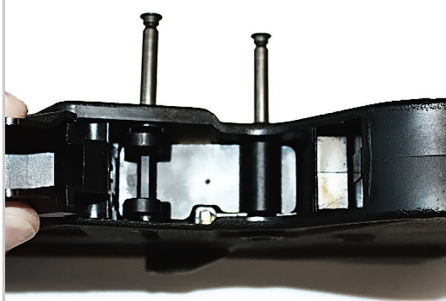
Pins out with open Bolt carrier lever
